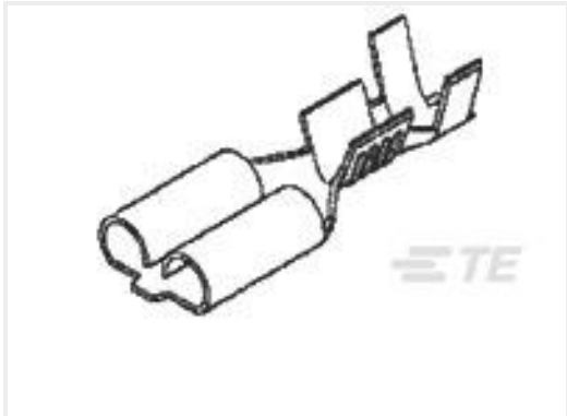
TE Part #170032-1 250 FASTON,REC.,20-14 AWG,BR
