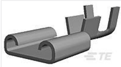
TE Part #4-160256-2 250 FASTON, REC., 17-14 AWG, PNST
