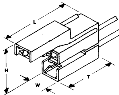
E .187 SERIES
