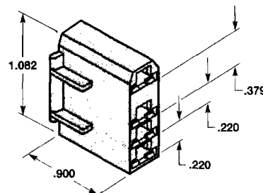
4 CIRCUIT .250 SERIES FASTON HOUSING
