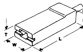
C .205/.187 SERIES
