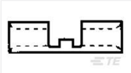
TE Part #323698 SPLICE,SOLIS BUTT HT 12-10
