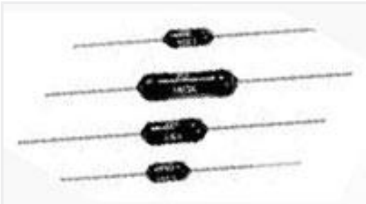
TE Part #9-1879678-4 H4 1K0 0.1% 50PPM
