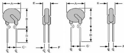
Fig.1 Lead Size : 24AWG Ø0.51 mm Diameter
