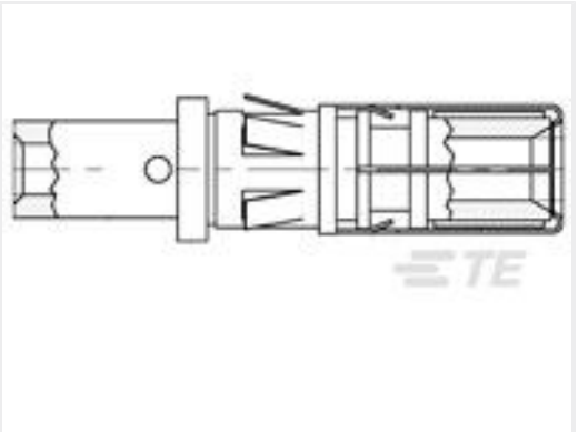
TE Part #202418-1 SKT CONT ASSY,TYPE I
