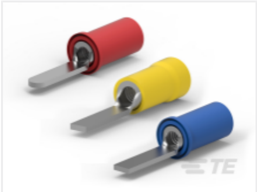
TE Part #CAT-P592-T116 PIDG Pre-Insulated Diamond Grip Tabs
