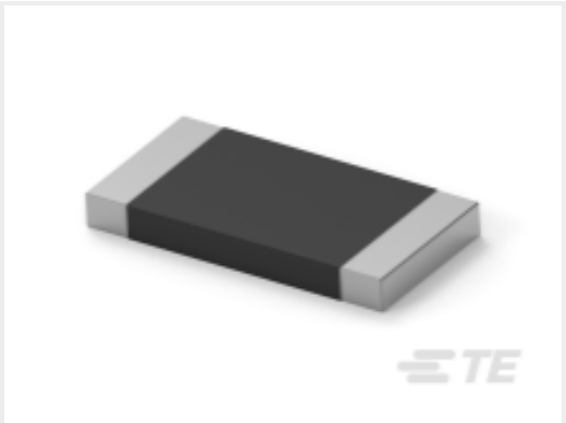
TE Part #6-2176422-2 TLRP 2512 3.0W R033 1% 50PPM 4K RL
