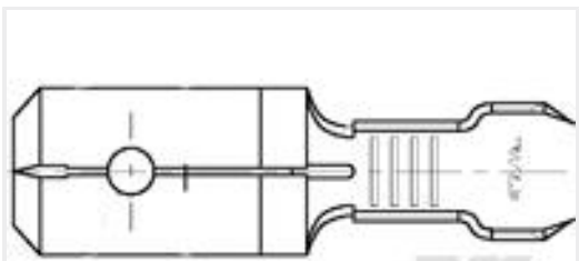
TE Part #42475-4 250 FASTON TAB 22-18 AWG TPBR
