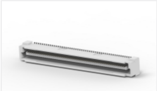
TE Part #CAT-313-PCB100 Free Height Plug Connector: Board- Board, Vertical, 100, 0.8mm
