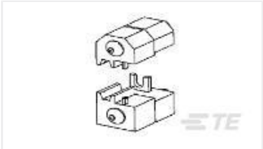
TE Part #90145-1 TYPE XII MALE FEMALE ASSY 14-12 DIE SET
