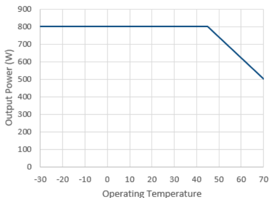
PQU1000; Convection Cooling
