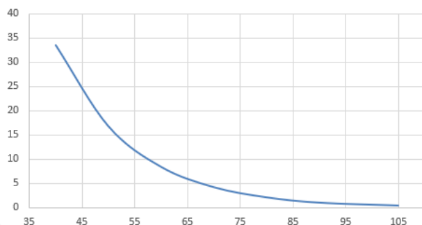
CB1 (PFC Bulk Cap) Life Predication
