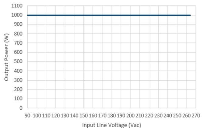
PQU1000 Forced Convection Cooling
