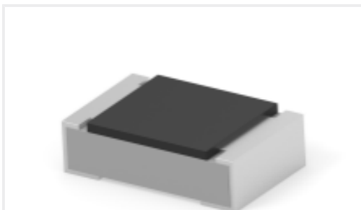
TE Part #7-2176569-8 RLC73K 2A R422 1% 5K RL
