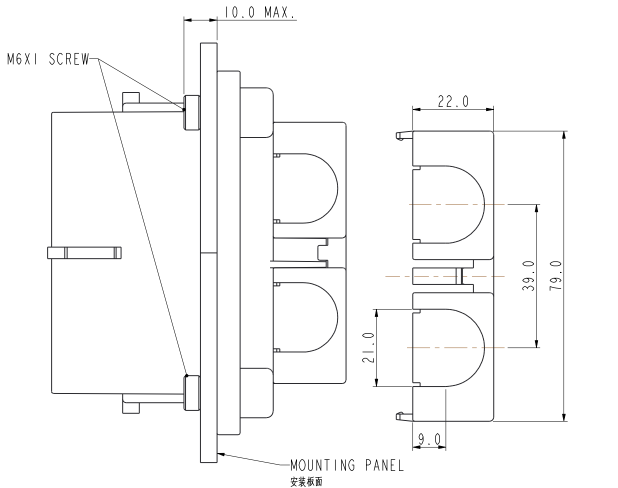
REAR MOUNTING SCREW SPECIFICATION 后安装 螺钉尺寸规格
