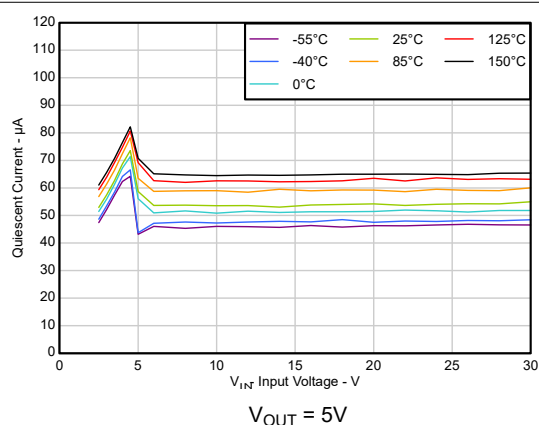
Figure 5-12. Quiescent Current vs Input Voltage ( I_L = 0 ) (New Chip)
