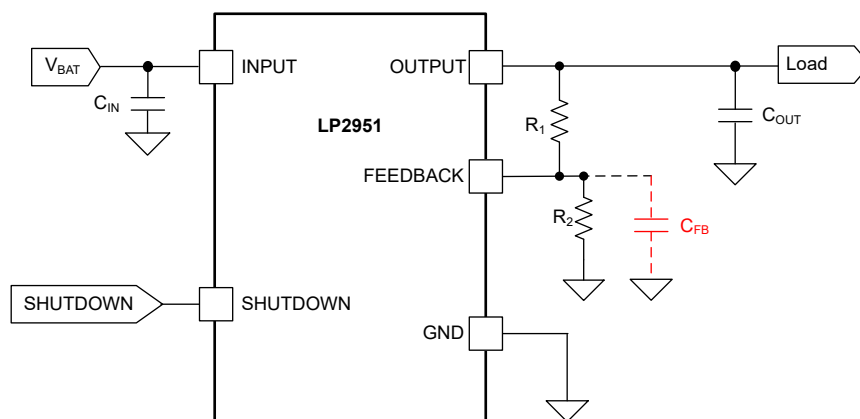
Figure 7-3. Formation of Parasitic Capacitor at the FEEDBACK Pin
