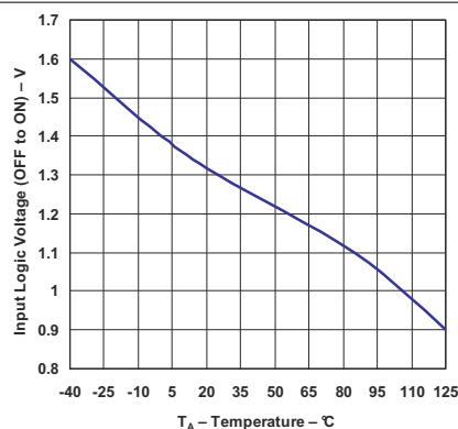
Figure 5-36. Shutdown Threshold Voltage (Off to On) vs Temperature (Legacy Chip)
