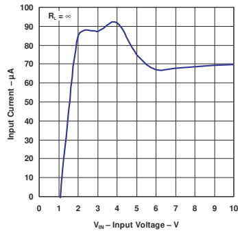
Figure 5-3. Input Current vs Input Voltage ( R_L = \text{OPEN} ) (Legacy Chip)
