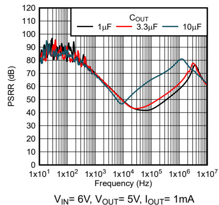
Figure 5-60. Ripple Rejection vs Frequency (New Chip)
