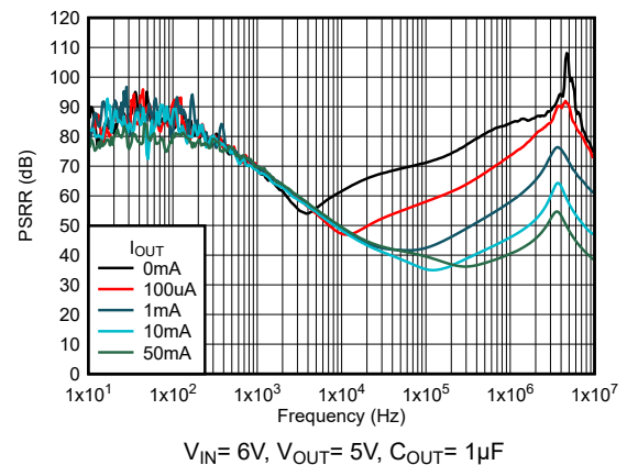
Figure 5-58. Ripple Rejection vs Frequency (New Chip)
