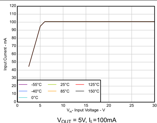
Figure 5-8. Input Current vs Input Voltage ( R_L = 50\Omega ) (New Chip)
