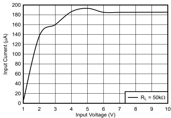
Figure 5-5. Input Current vs Input Voltage ( R_L = 50\text{k}\Omega )
