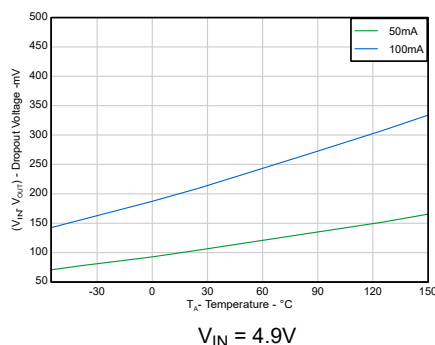
Dropout Voltage vs Temperature (New Chip)
