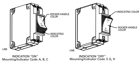
INDICATION "ON"
