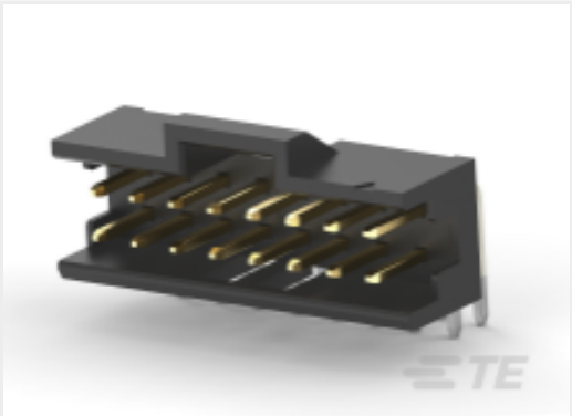
TE Part #2-2823411-0 20P,2MM,PL HDR,DRRT,2.8,0.76AU,TB
