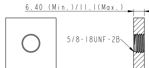
Panel cut out (screw type)
