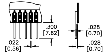
LS pc board w/solder pins
