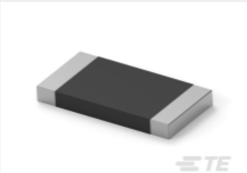
TE Part #3-2176421-3 TLRP 2512 2.0W R080 1% 25PPM 4K RL
