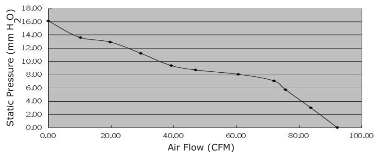
CFM-9238S-250-532
