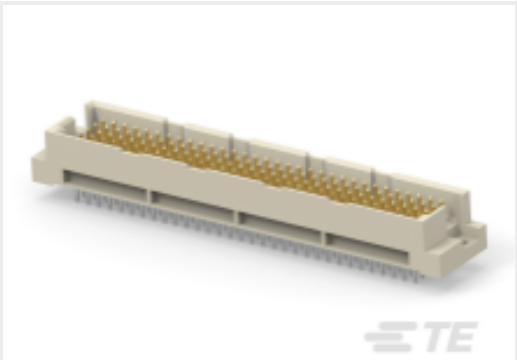
TE Part #374472-E STVTE 160 MI ABCDE VVVV 4-00 GA06 4,0 *
