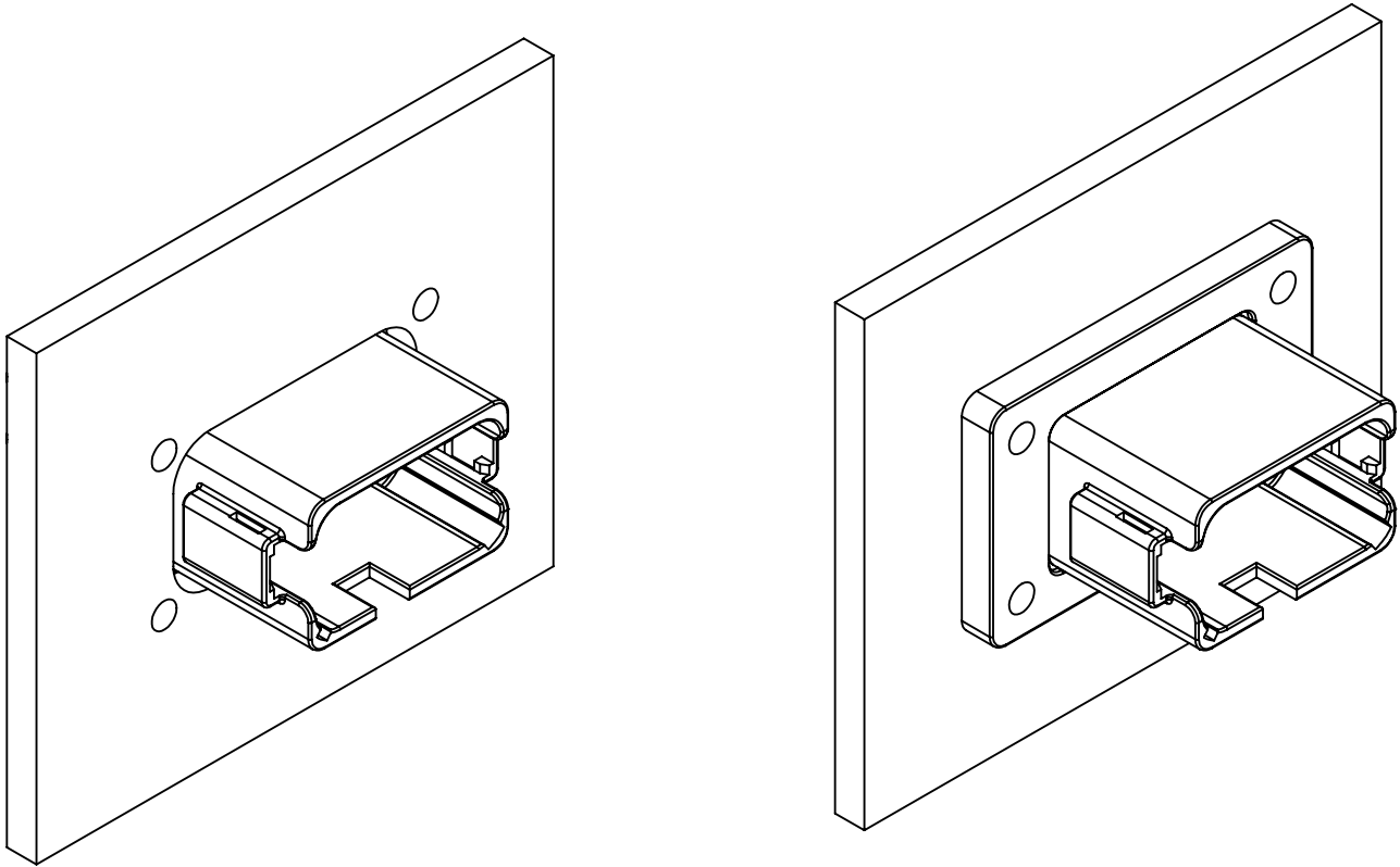
FRONT MOUNT
