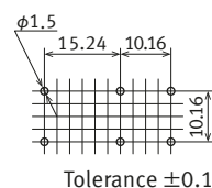
Recommended PC board pattern ( BOTTOM VIEW )
