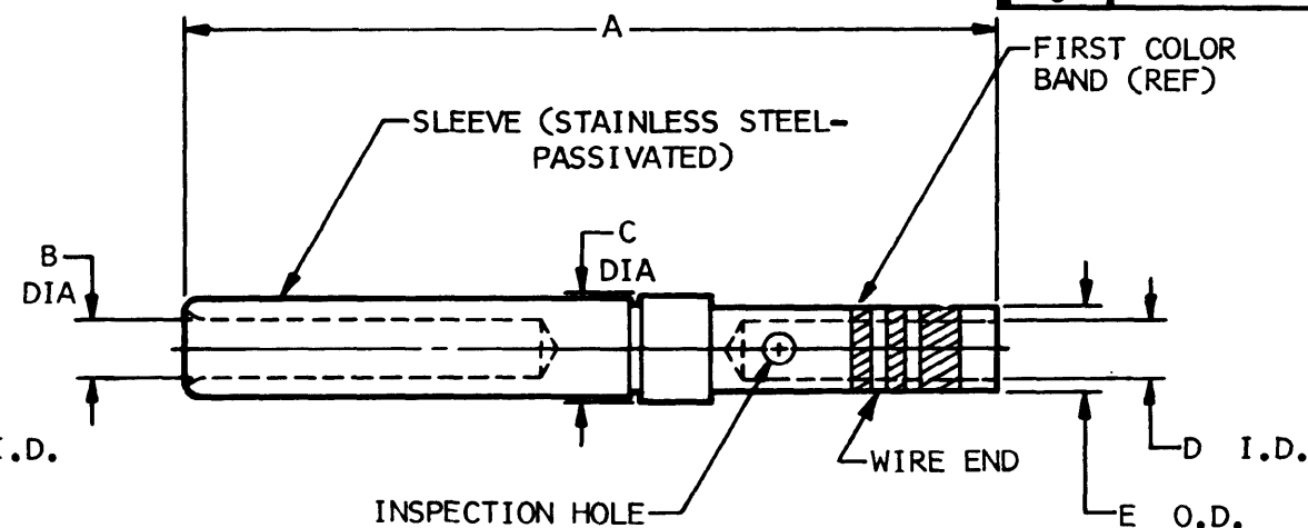
SOCKET CONTACT (EXAMPLE)
