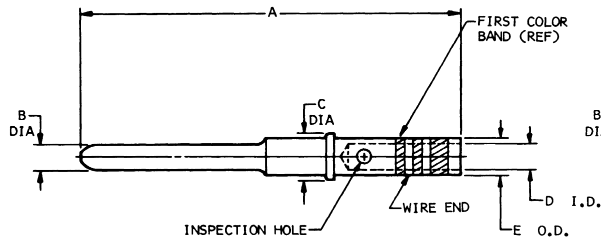
PIN CONTACT (EXAMPLE)
