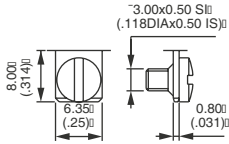
Screw ( standard)
