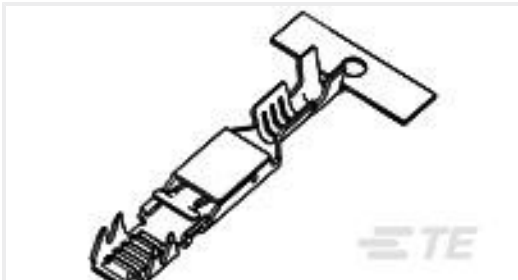
TE Part #353842-1 FPC SENSOR CONT.
