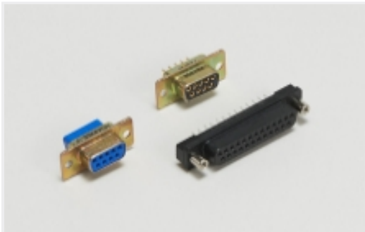
D-Shaped Connectors(234)
