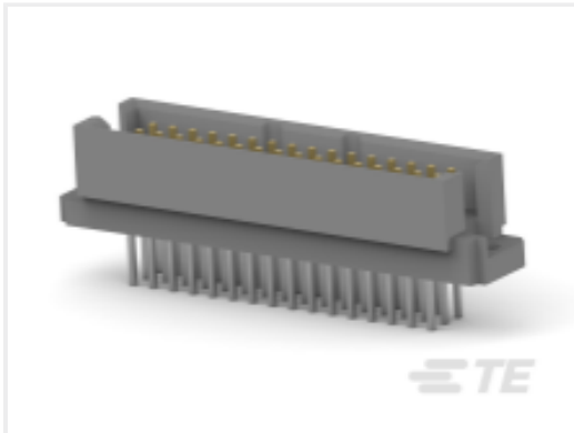
TE Part # 5650918-5 ASSY,PIN,EUROCARD,TYPE R/2,LEA
