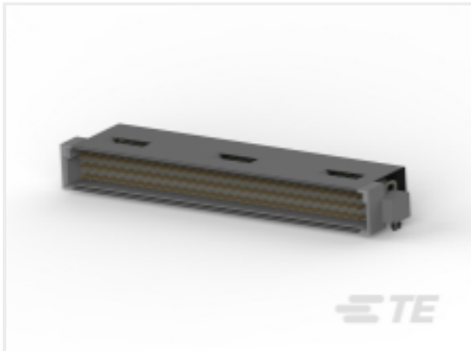
TE Part # 5536148-5 ASSY,PIN,ENH.TYPE C,EUROCARD,L- FREE,5ROW
