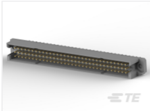
TE Part # 5536019-5 ASSY,PIN,EUROCARD,TYPE R,LEAD- FREE,96 PO
