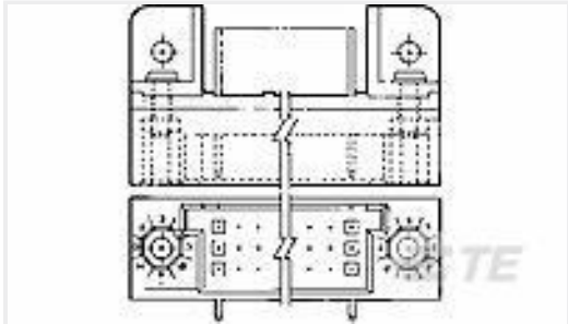
TE Part #533288-7 HDI PIN ASSY 3 ROW 150 POS R/A
