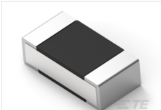
TE Part #8-2176307-8 RP 1E 0.1W 100K 0.1% 25PPM 5K RL
