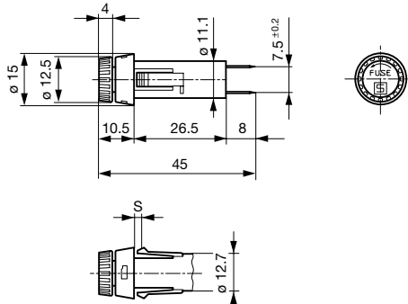
Variants Fingergrasp 3101.0035, 3101.0235, 3101.0036 and 3101.0336 s = Panel thickness (see variants)
