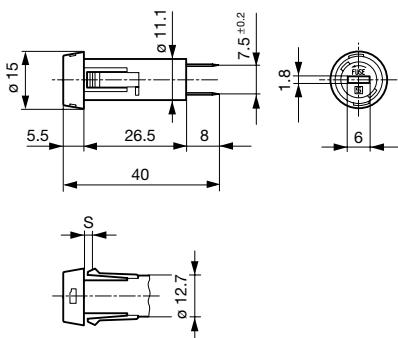
Variants 3101.0030, 3101.0230, 3101.0031 and 3101.0331 s = Panel thickness (see variants)
