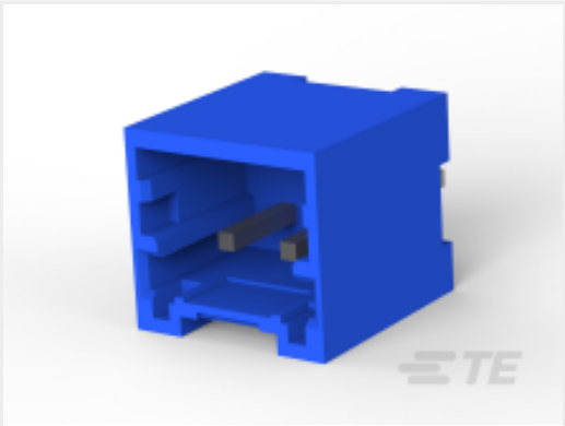
TE Part #2-1971032-2 2POS HEADER ASSEMBLY FOR GIC 2.0 EV
