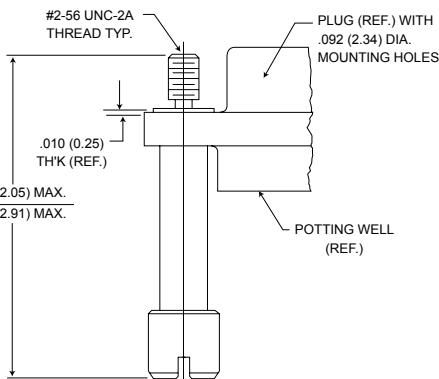
Figure 2. Jackscrew - High Profile Slotted Head Size 9-69 Size 100*
