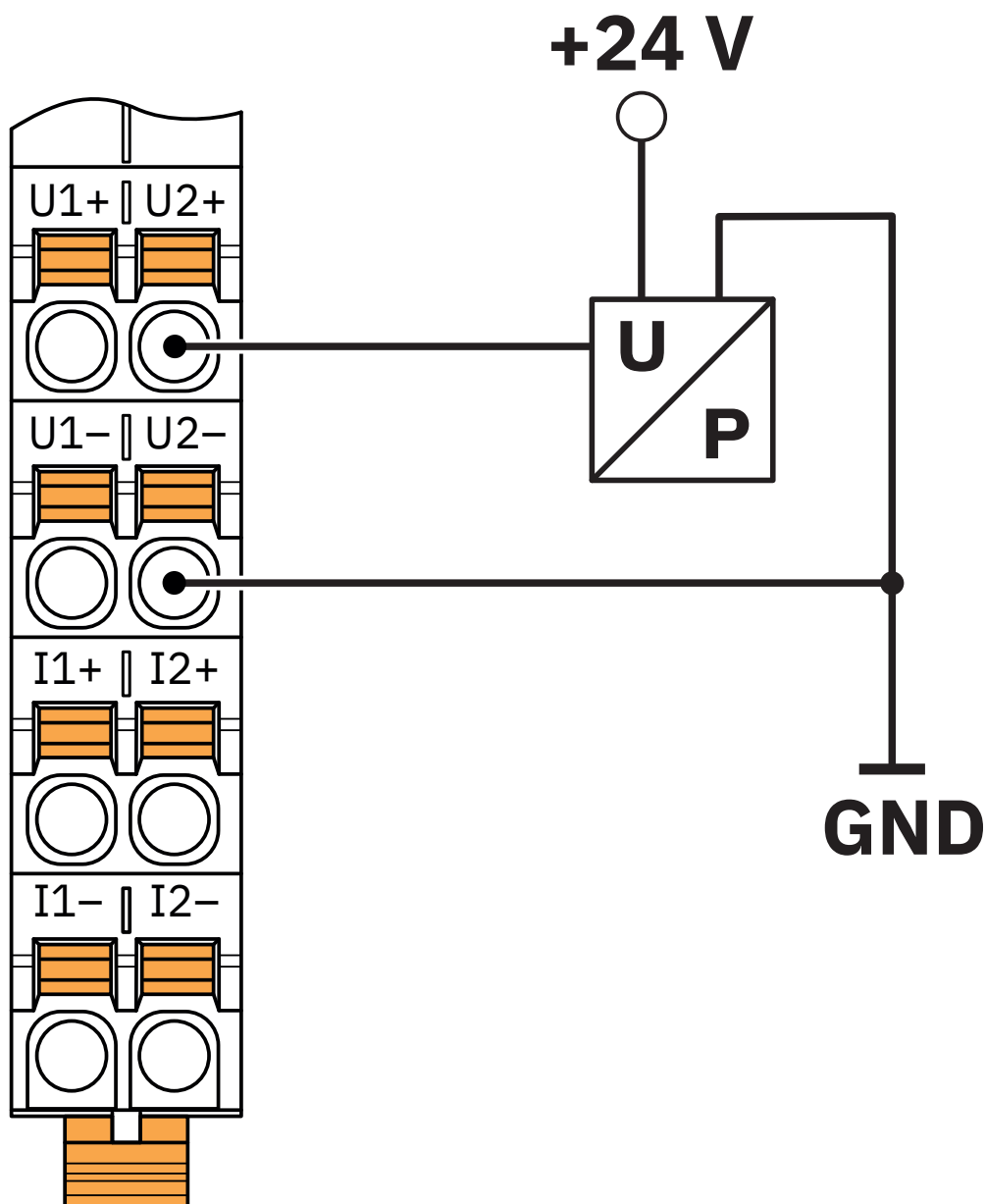
Connection diagram
