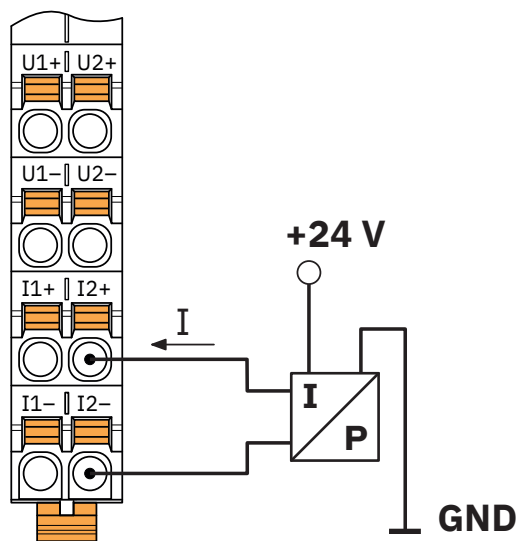
Connection diagram
