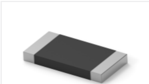
TE Part #3-2176422-2 TLRP 2512 3.0W R050 1% 25PPM 4K RL
