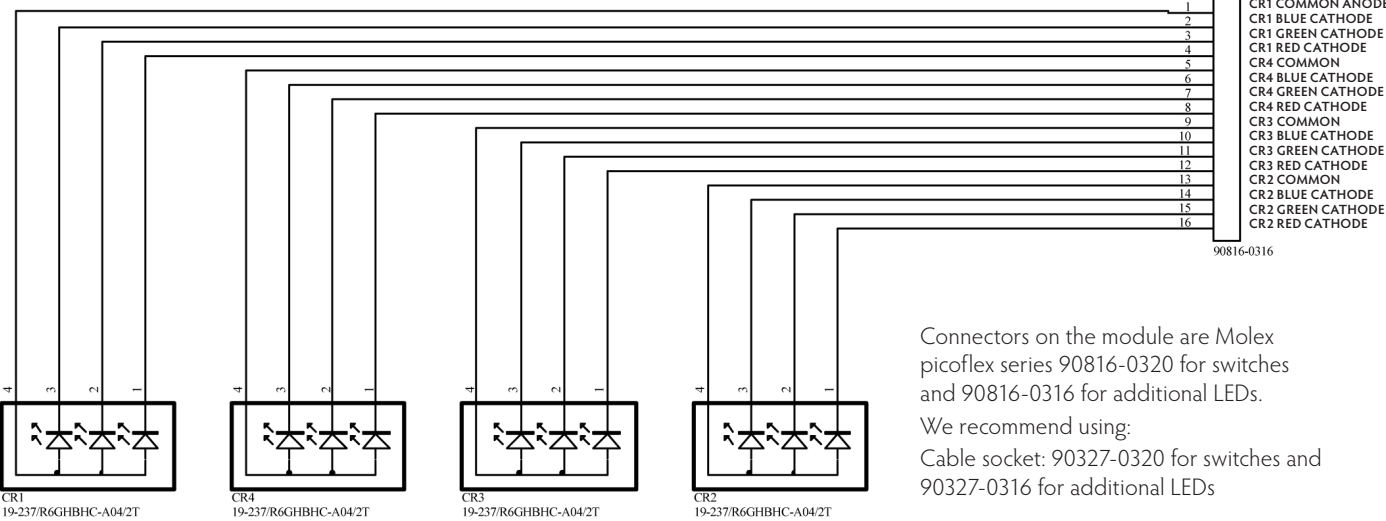
Circuit diagram for additional LEDs for controlmec™
