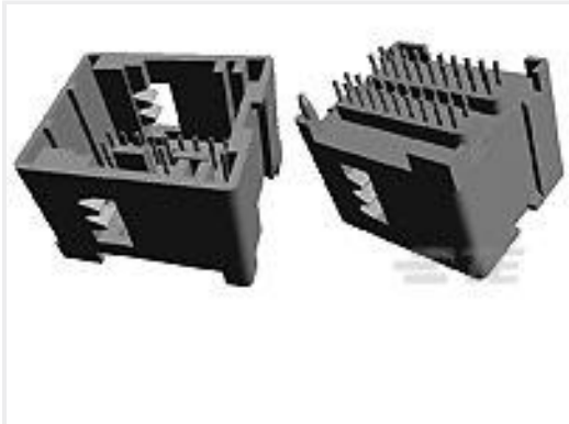
TE Part #953118-1 40pos MQS .63 header 180deg
