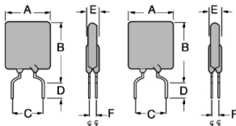
Fig.3 Lead Size : 20AWG Ø 0.81 mm Diameter
