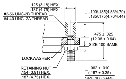
Figure 3. Jackpost Assembly Size 9-69 Size 100*
