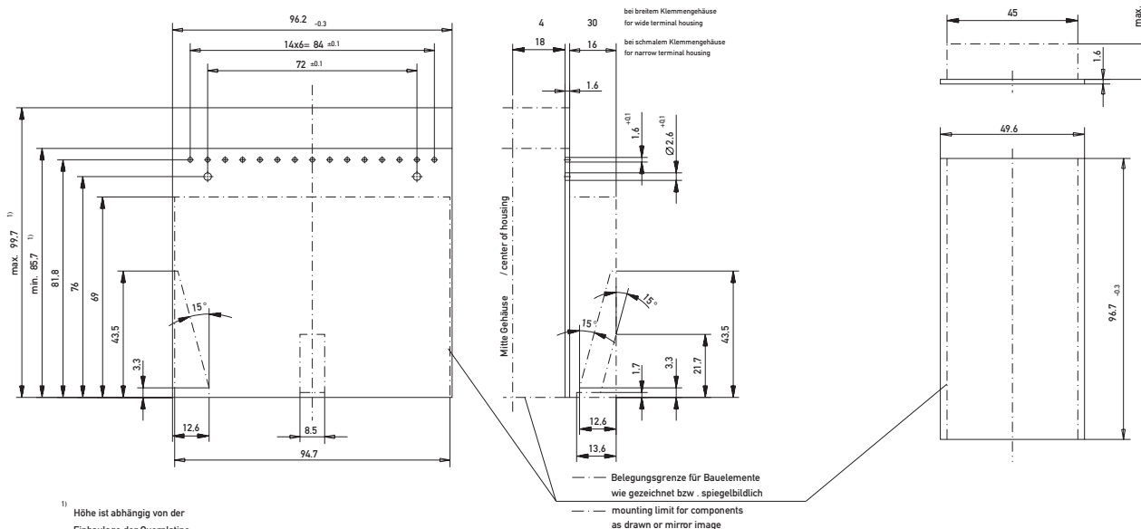
Querplatine / Crosswise circuit board
